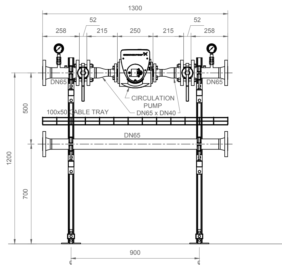
ELEVATION VIEW
