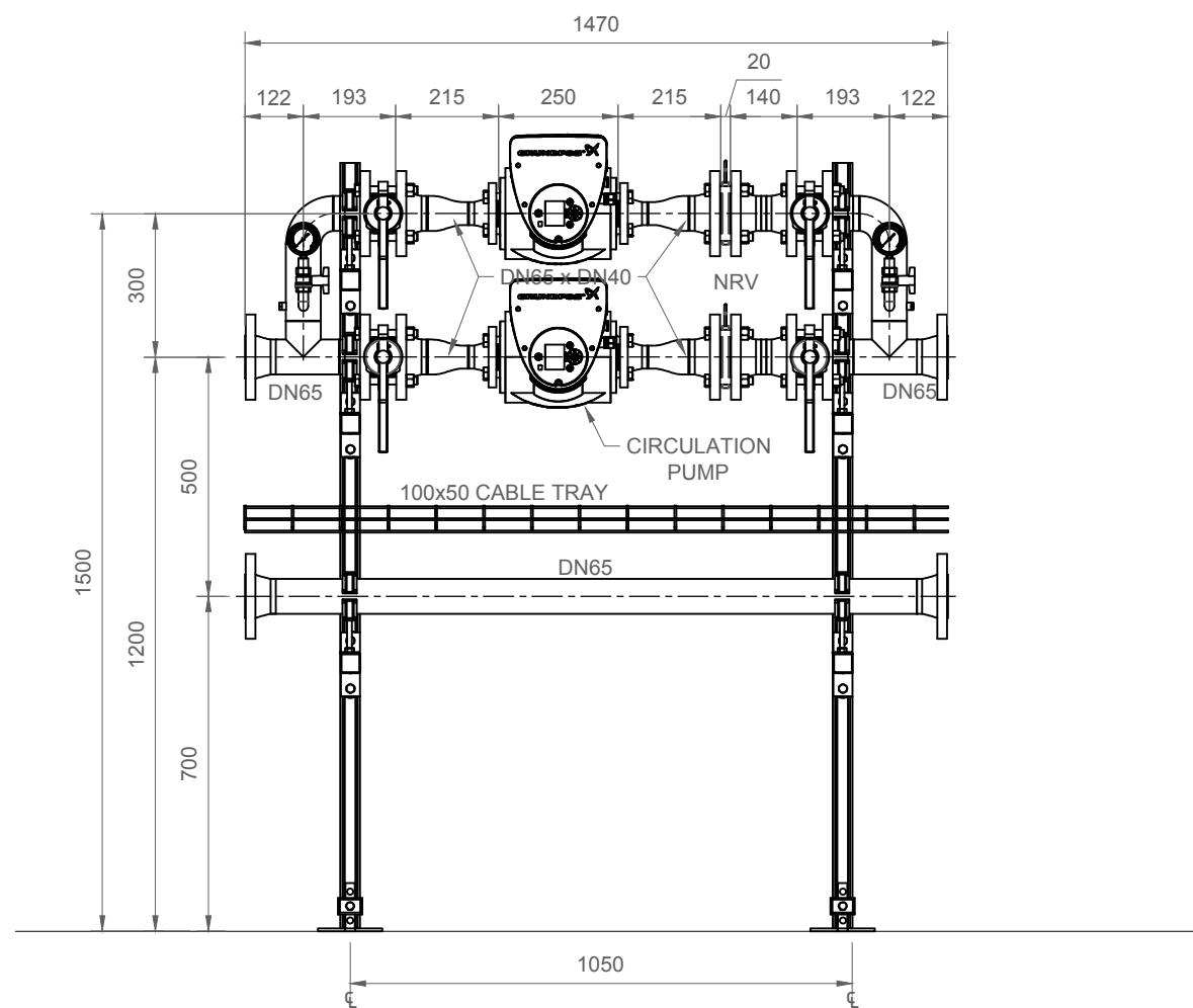
ELEVATION VIEW
