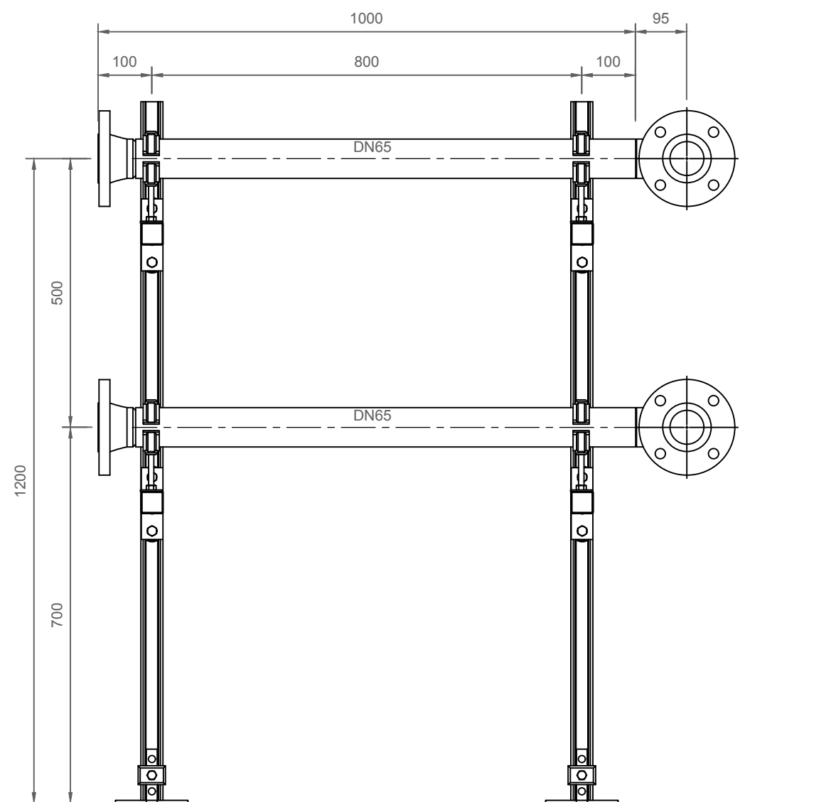
ELEVATION VIEW
