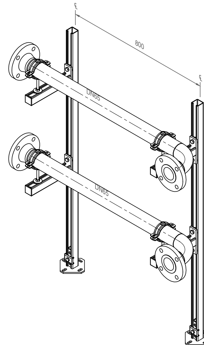
ISOMETRIC VIEW
