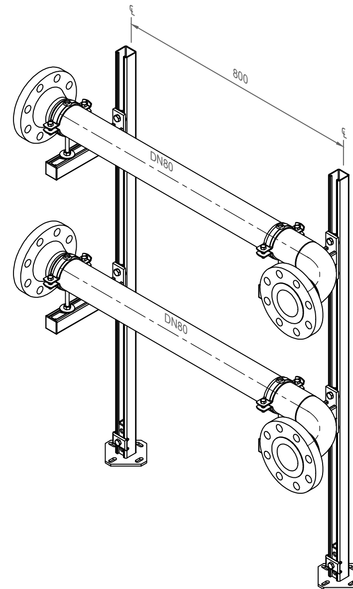
ISOMETRIC VIEW
