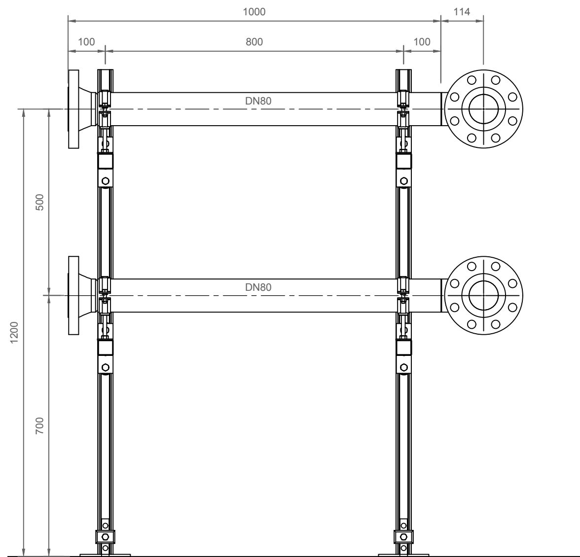
ELEVATION VIEW
