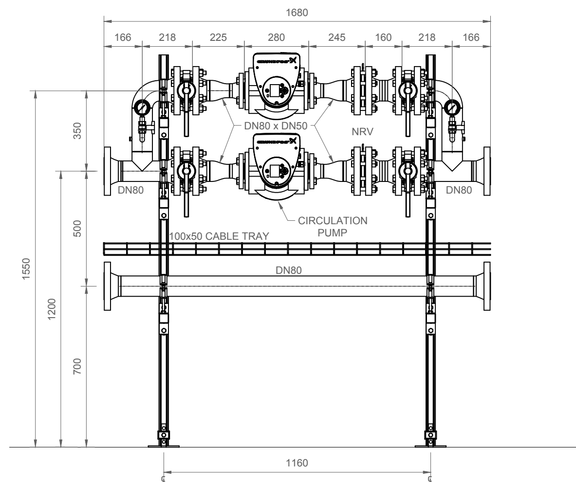
ELEVATION VIEW
