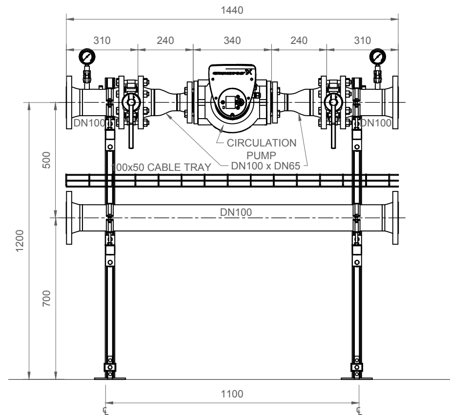
ELEVATION VIEW
