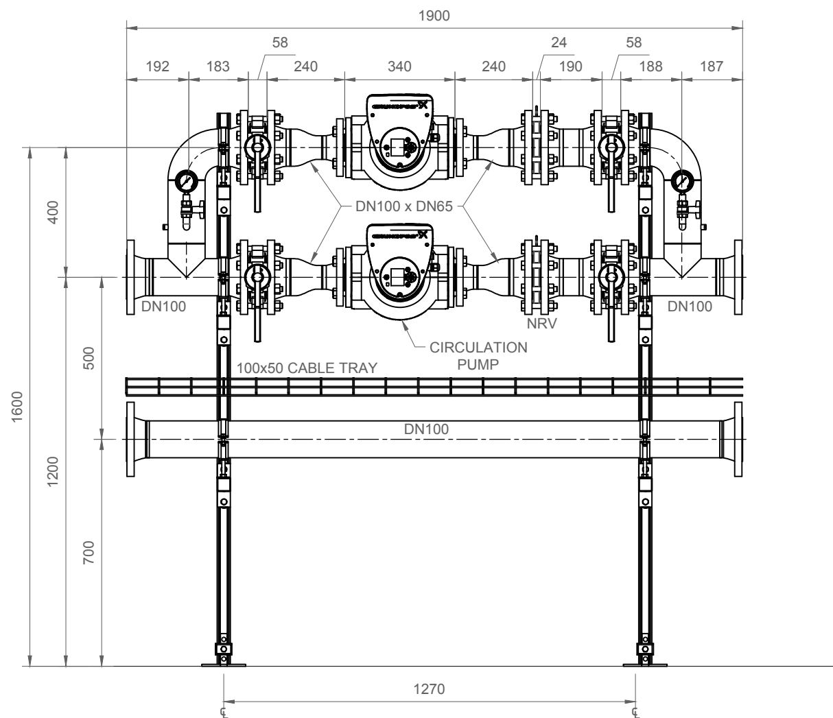
ELEVATION VIEW
