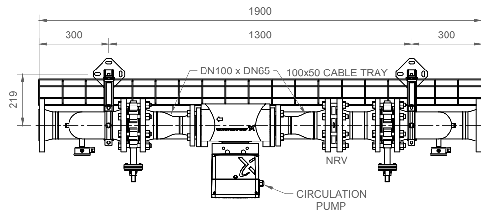
PLAN VIEW
